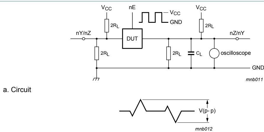
Fig. 17. Test circuit for measuring crosstalk voltage (between the digital input and the switch)
